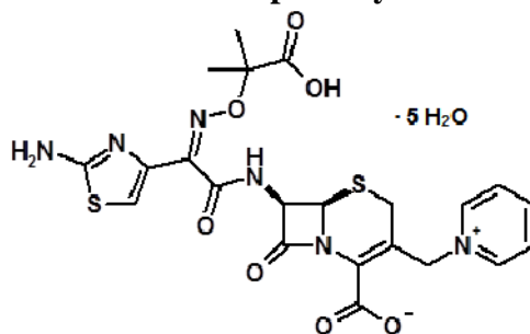
Figure 1 Chemical structure of ceftazidime pentahydrate
