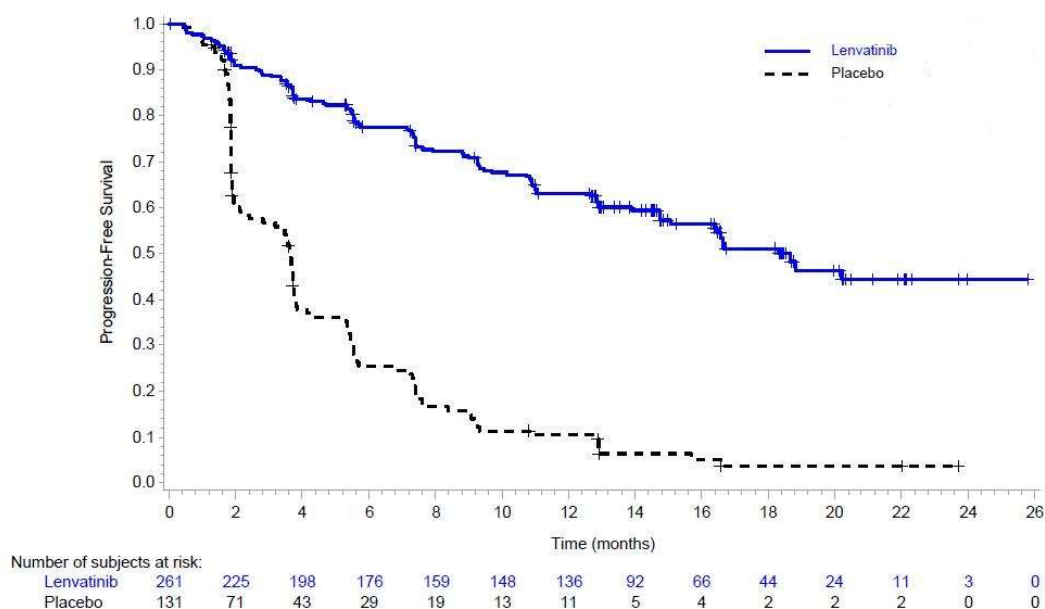
Figure 1: Kaplan-Meier Curves for Progression-Free Survival in SELECT
