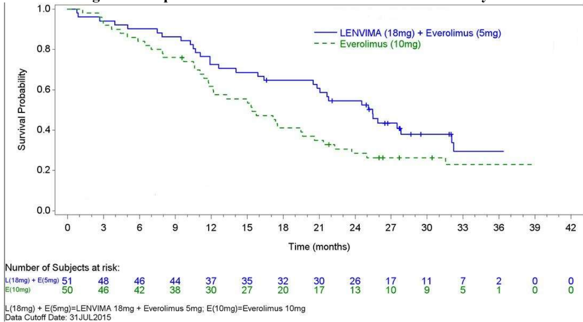
Figure 5: Kaplan-Meier Curves for Overall Survival in Study 205
