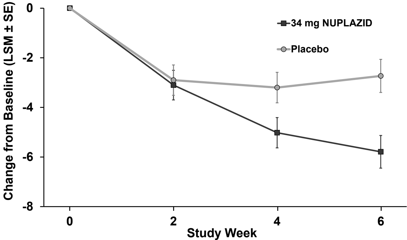
Figure 3 SAPS-PD Change from Baseline through 6 Weeks Total Study Treatment
