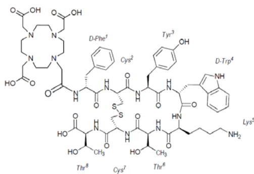
Figure 2 Chemical Structure of dotatate
