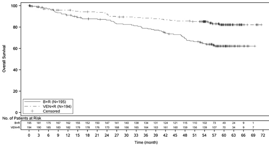
Figure 4. Kaplan-Meier Curve of Overall Survival in MURANO
