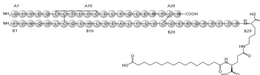
Figure 1. Structural Formula of Insulin degludec
