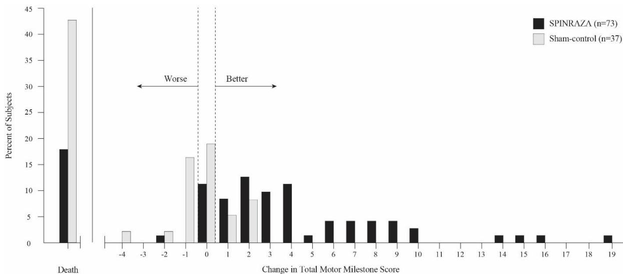
Figure 1. Percent of Patients Who Died and Net Change from Baseline in Total Motor Milestone Score (HINE) Among Patients Alive in the Final Efficacy Set of Study 1 *
