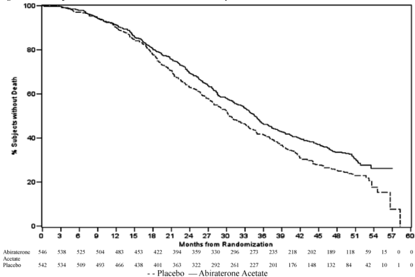
Figure 2: Kaplan Meier Overall Survival Curves in Study 2
