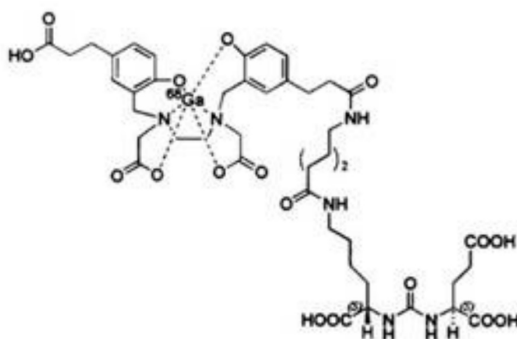
Figure 1: Chemical Structure of Gallium Ga 68 Gozetotide
