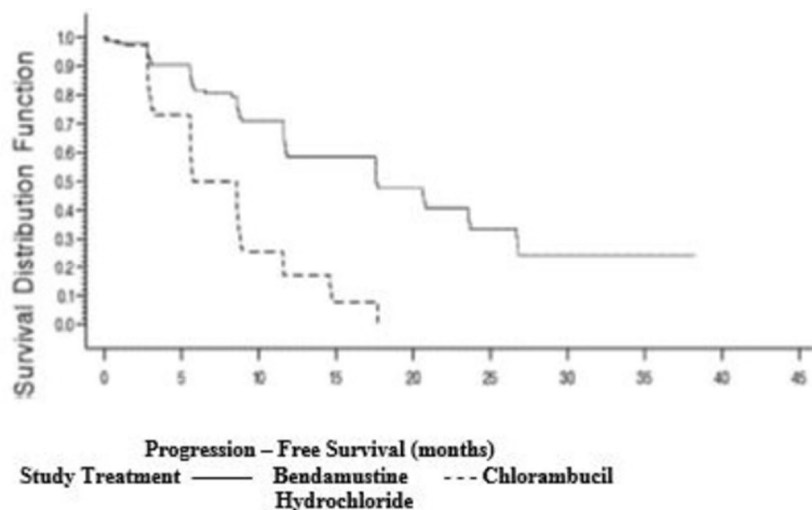
Figure 1. Progression-Free Survival
