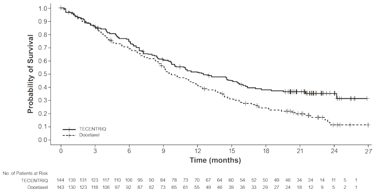
Figure 2: Kaplan-Meier Plot of updated Overall Survival in Study 3
