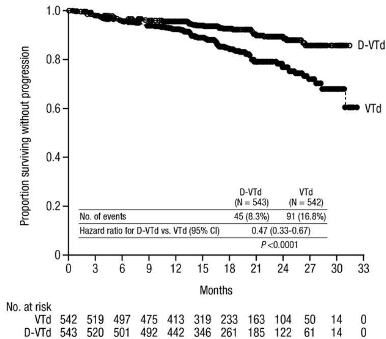
Figure 4: Kaplan-Meier Curve of PFS in CASSIOPEIA a
