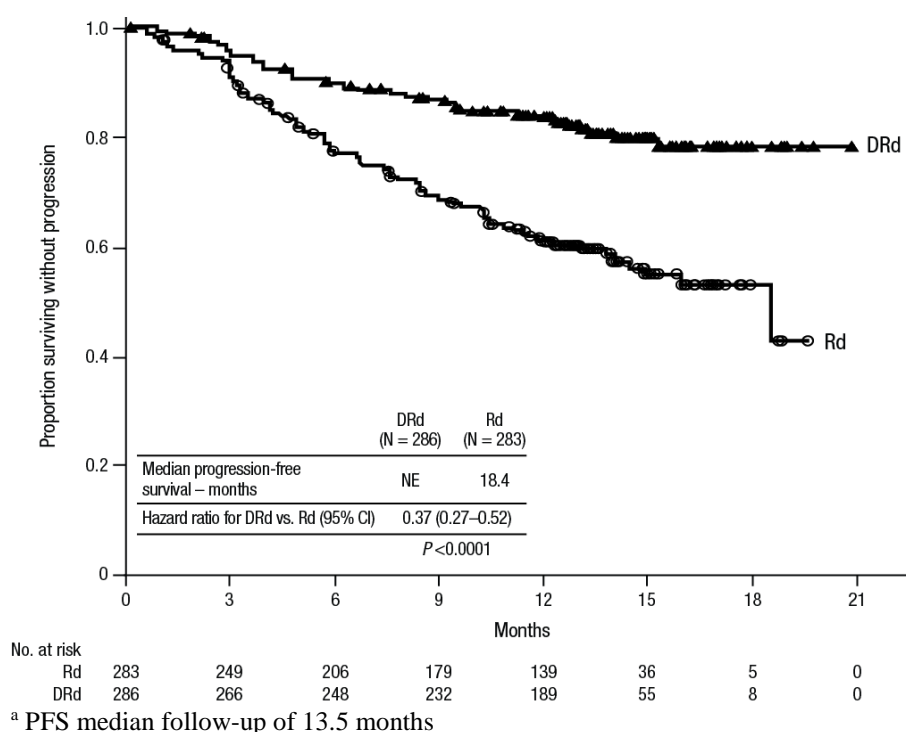
Figure 5: Kaplan-Meier Curve of PFS in POLLUX a
