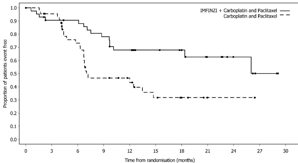
Figure 6. Kaplan-Meier curve of PFS for Patients with dMMR Tumors in DUO-E
