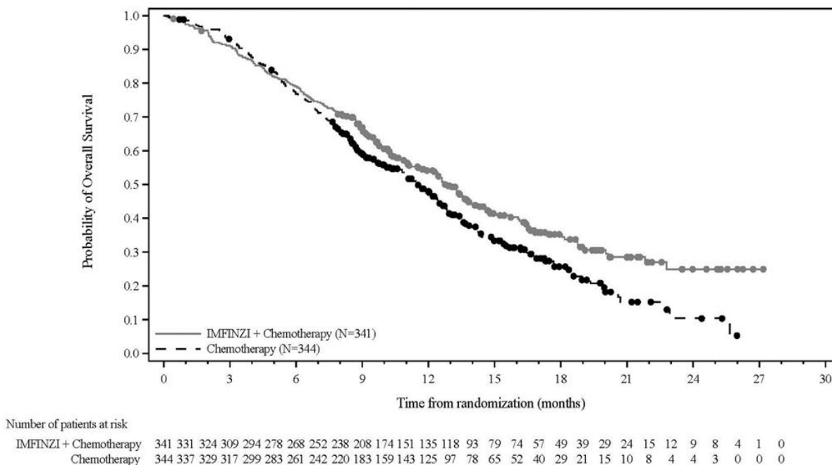
Figure 4: Kaplan-Meier Curve of OS in TOPAZ-1 Study
