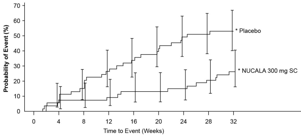
Figure 4. Kaplan-Meier Curve for Time to First Hypereosinophilic Syndrome Flare
