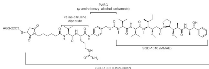
Figure 1. Structural Formula
