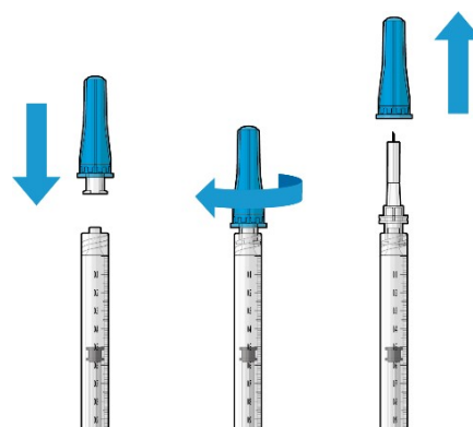
Figure 14 Initial fill needle attached to syringe and cap removal
