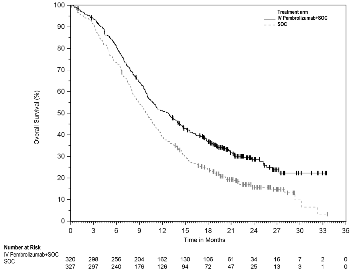
Figure 22: Kaplan-Meier Curve for Overall Survival in KEYNOTE-590 (CPS ≥1)
